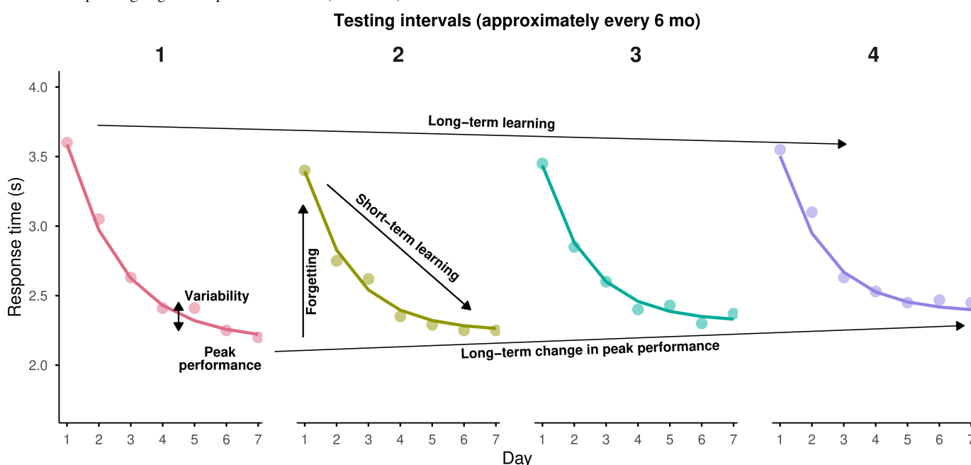
Figure 2. Illustration of the Bayesian double-negative exponential model with 4 testing intervals for 1 synthetic participant. Data are displayed as dots. Corresponding negative exponential curves (solid lines) show model fit.
